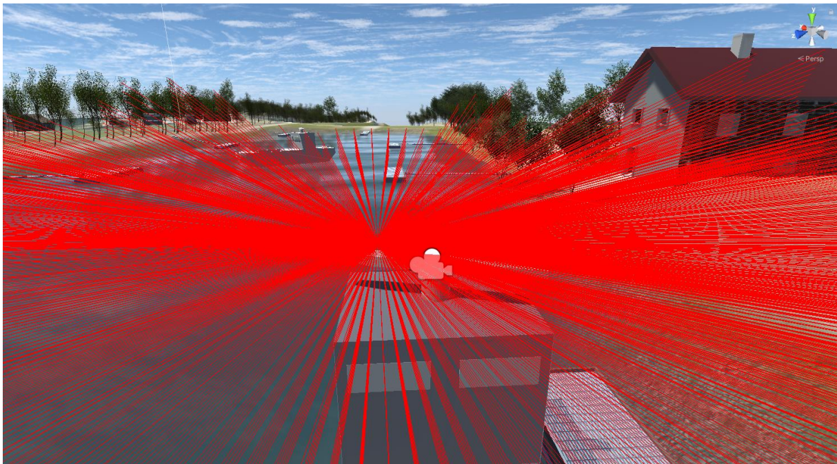
Fig 1. Unity3d scene with visualization of reflected RADAR rays.
